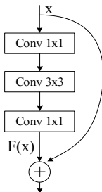
Figure 2. The classic residual block.
