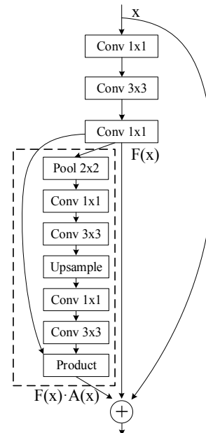
Figure 3. Attention-based residual block.
